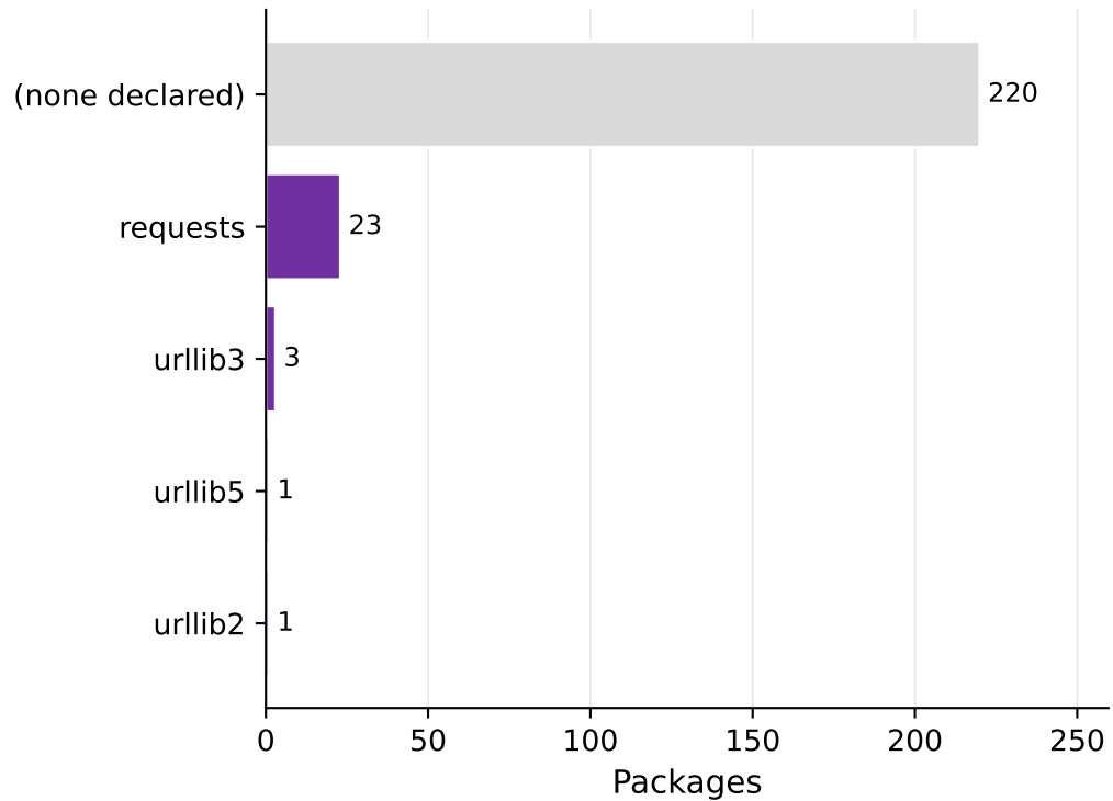
Declared install-time prerequisite
